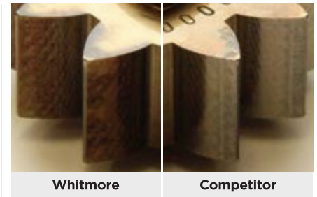
Figure 1: Gears showing FZG testing results. Both of the above FZG gears have been used to test lubricants that passed 12 stages and then been through the 30-hour Extended Wear Test. The gear on the left was used when testing Envirolube XE Extreme, and the original crosshatch pattern on the gear is still clearly visible. The gear on the right is more typical, as the crosshatch has been partially worn off. This test often shows scuffing, but in this case, the damage has been done by a form of wear called polishing.
